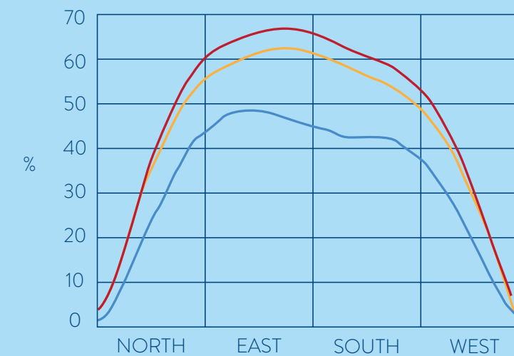
Reduction in primary energy use for heating, cooling and lighting through shading, when compared to the energy use without shading, for double glazing (red), low-e glazing (orange), and solar control glazing (blue).
